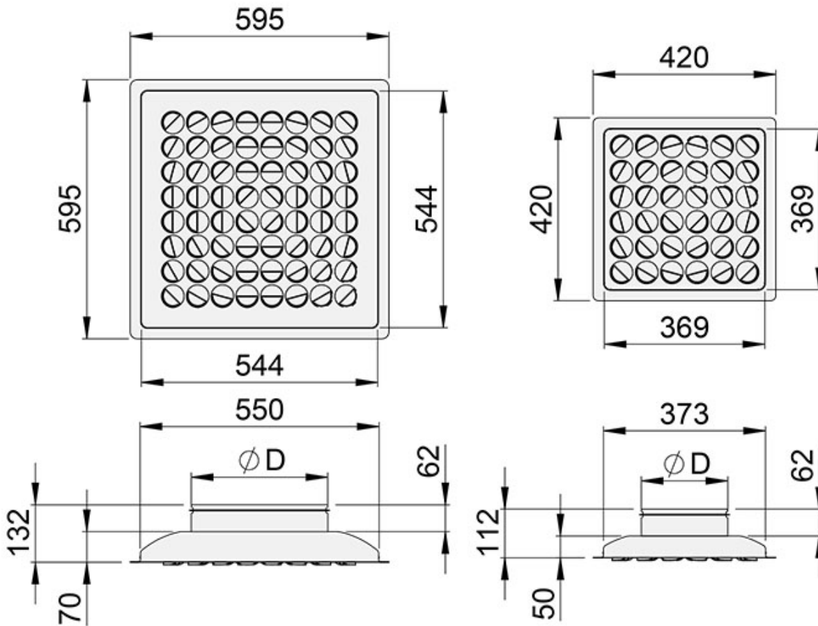
Fig. 4. Dimensions of Halton Jaz JSC diffuser, 600×600 mm (left) and 420×420 mm (right)
