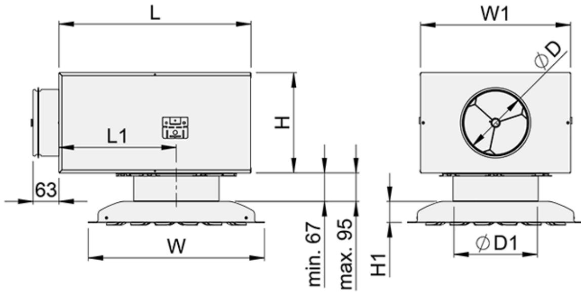
Fig. 5. Halton Jaz JSC with Halton Pop PDI plenum, externally positioned connection spigot
