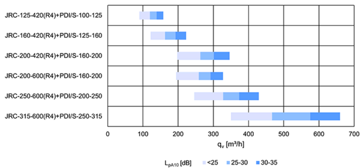
Fig. 4. Quick selection with unit m³/h
