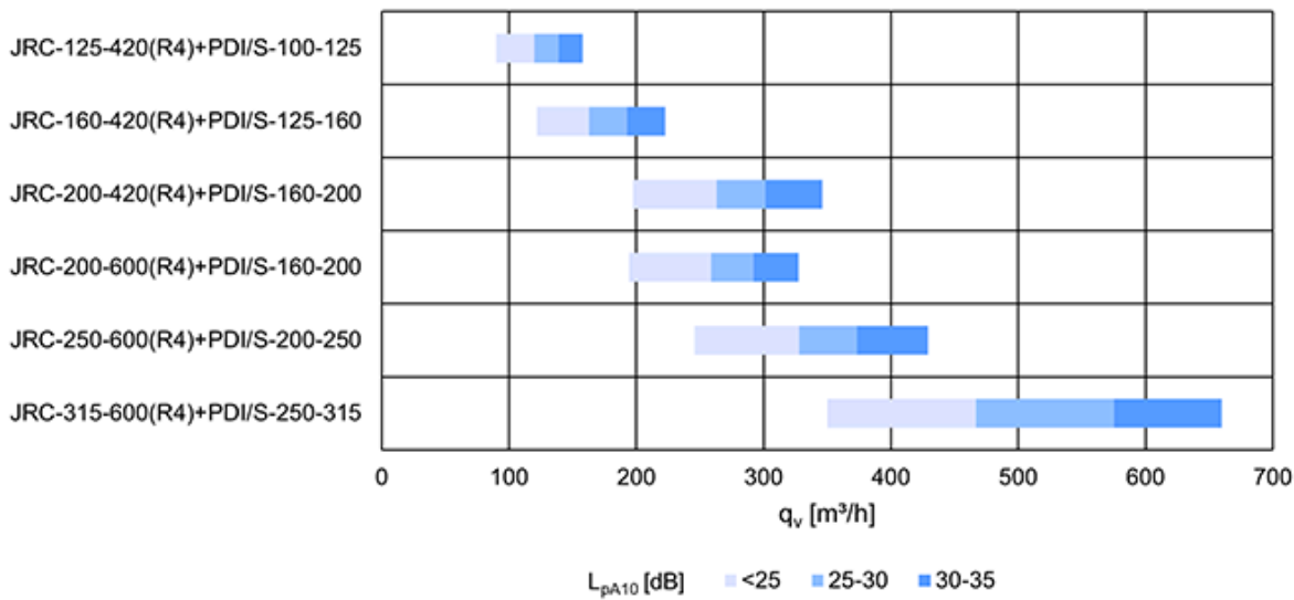
Fig. 4. Quick selection with unit m 3 /h
