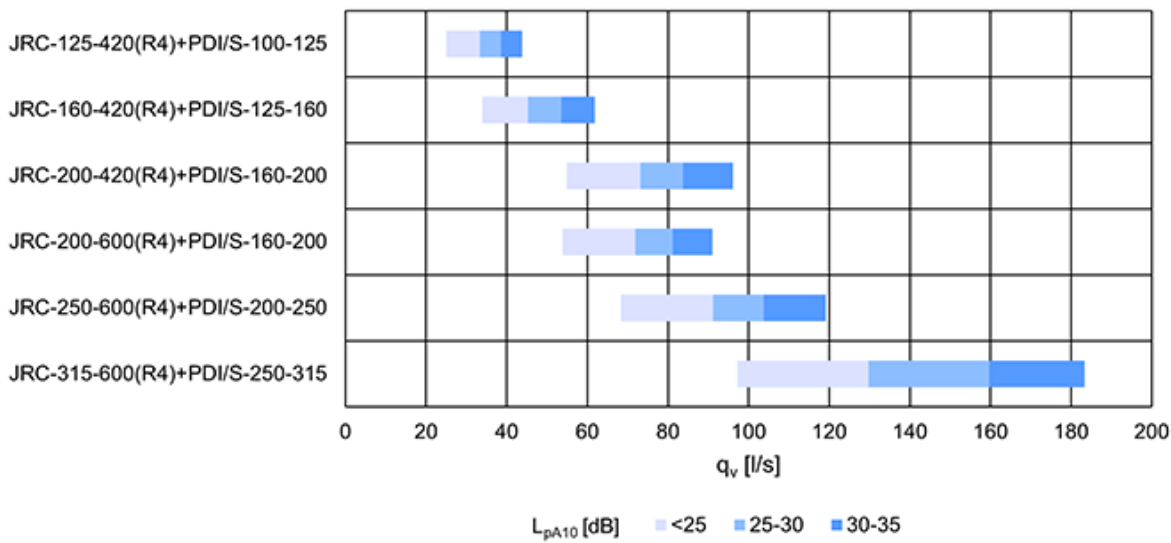
Fig. 3. Quick selection with unit l/s
