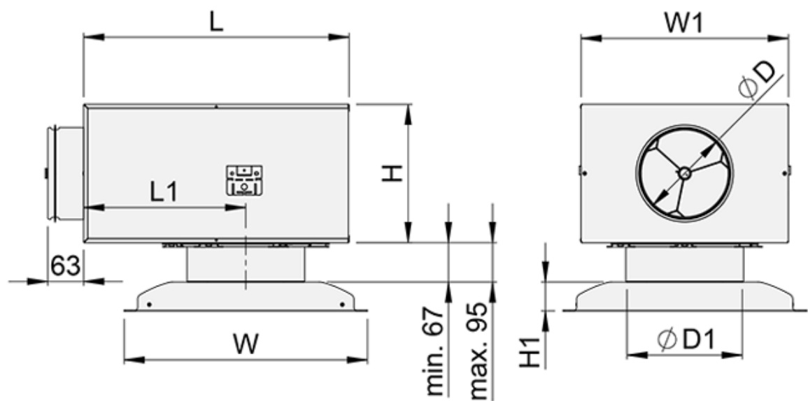
Fig. 6. Halton Jaz JRC with Halton Pop PDI plenum, externally positioned connection spigot
