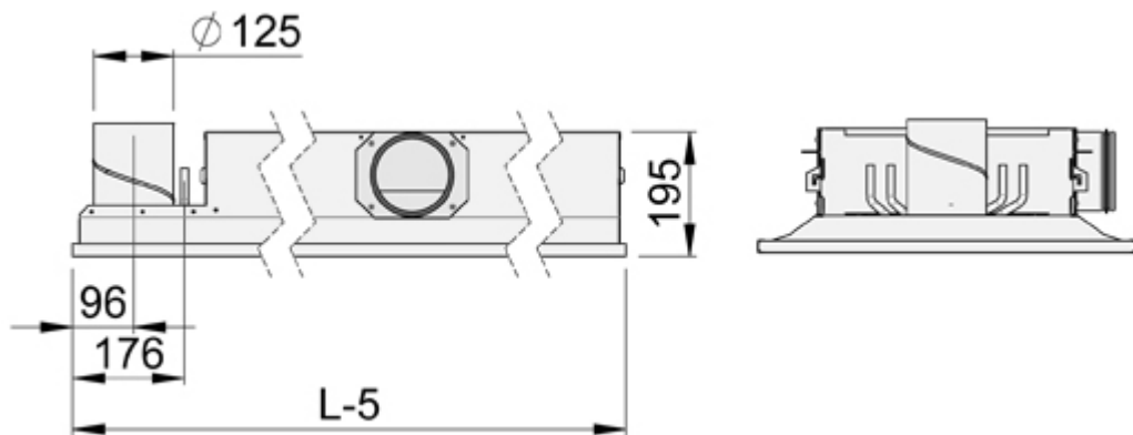
Model with integrated exhaust (EX=A)
