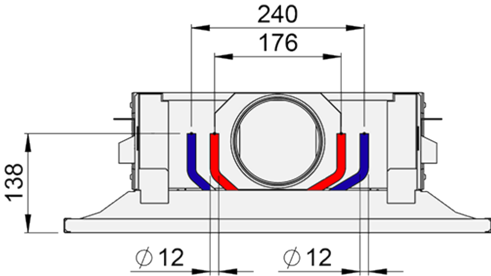
High efficiency coil, twin loop (CE=H2)
