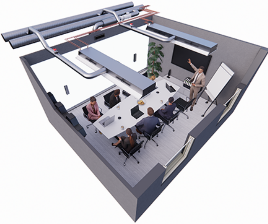
Fig. 2: Halton Rex 600 (RE6) active chilled beams with HAQ control and PTS damper, controlled with Halton Workplace WRA room automation controllers in a meeting room
