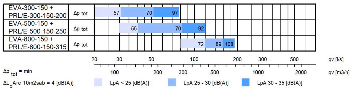
Fig.2. With Halton PRL plenum
