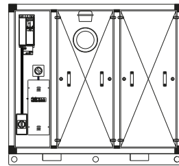
Light with switch and porthole options
