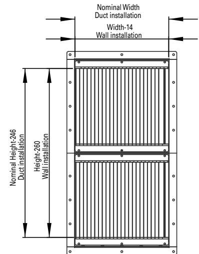
DSH MODULE UNIT (HEIGHT)
