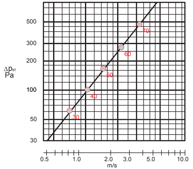
DSH stainless steel with mask louvre and ePM2,5 65% bag filter (measured size 1000 x 1000 mm)
