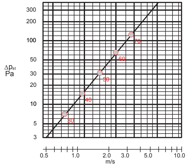
DSH stainless steel with mask louvre and ISO Coarse 70% panel filter
